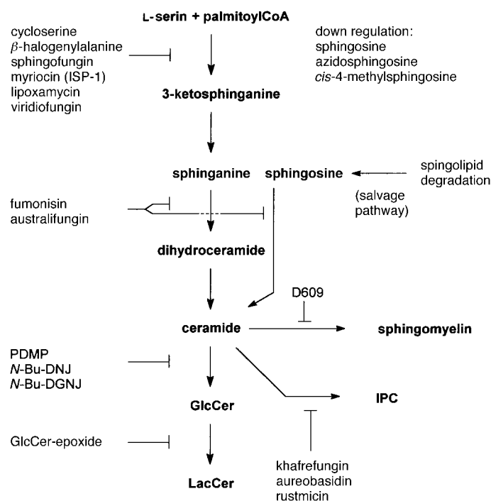
Figure 10. Flow scheme and inhibitors of sphingolipid biosynthesis (modified from reference [100]). IPC = inositolphosphorylceramide; N-Bu-DNJ = N-butyldeoxyonojirimycin; N-Bu-DGNJ = N-butyldeoxygalactonojirimycin; PDMP = 1-phenyl-2-decanoylamino-3-morpholinopropan-1-ol.
